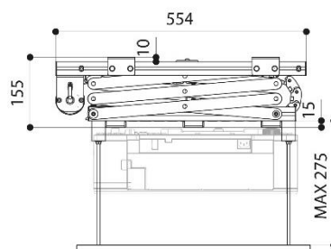
Frontal view closed
