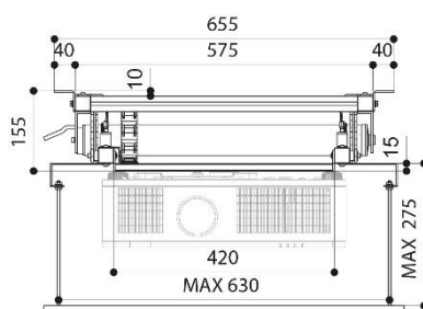
Side view closed
