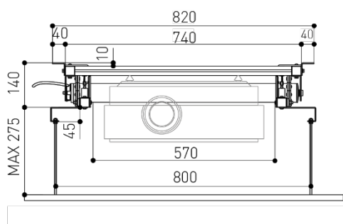
Vue de face fermée Frontal view closed
