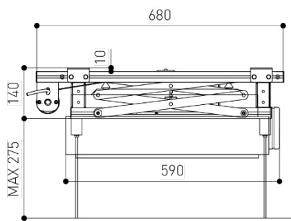
Vue latérale fermée Side view closed
