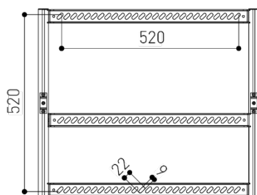
Distance max. des points de fixation VP Max. size projector anchoring points
